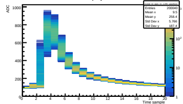
Run 045 Vol 1.28V | Crystal 12 SiPM 11
