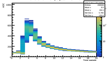
Run 045 Vol 1.28V | Crystal 12 SiPM 6
