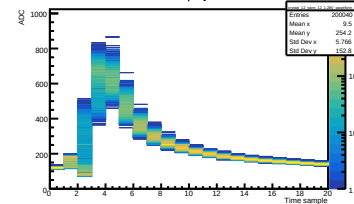
Run 045 Vol 1.28V | Crystal 12 SiPM 12
