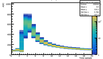
Run 045 Vol 1.28V | Crystal 12 SiPM 14
