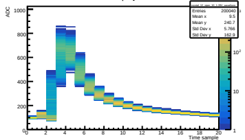
Run 045 Vol 1.28V | Crystal 12 SiPM 10
