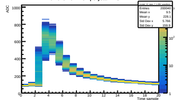
Run 045 Vol 1.28V | Crystal 12 SiPM 7
