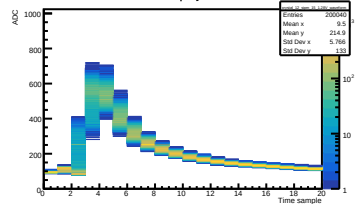
Run 045 Vol 1.28V | Crystal 12 SiPM 15
