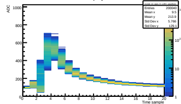
Run 045 Vol 1.28V | Crystal 12 SiPM 9
