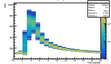
Run 045 Vol 1.28V | Crystal 12 SiPM 5
