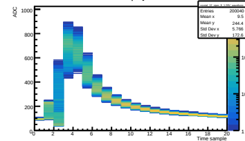
Run 045 Vol 1.28V | Crystal 12 SiPM 8
