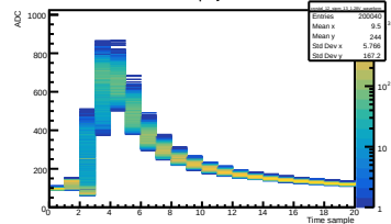
Run 045 Vol 1.28V | Crystal 12 SiPM 13
