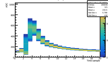
Run 045 Vol 1.28V | Crystal 12 SiPM 4
